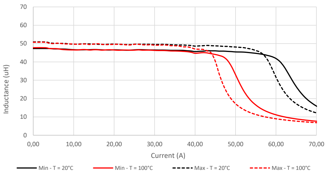
Figure 5. Inductance vs. DC bias @20°C and @100°C
