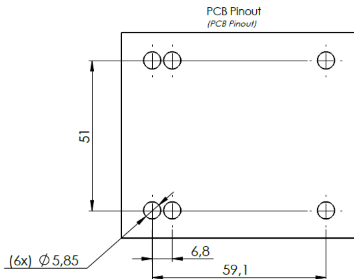
Figure 4. PCB Pinout
