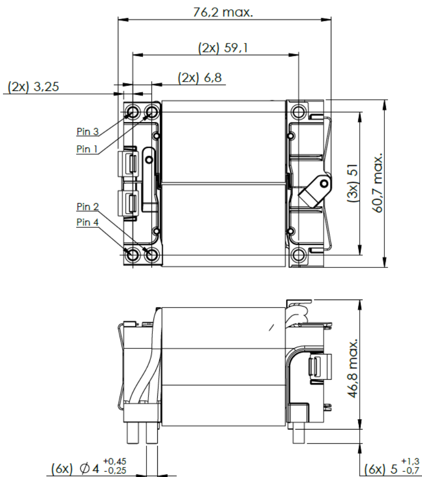
Figure 3. DC choke dimensions in mm
