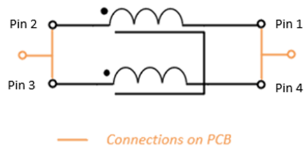
Figure 2. Electrical circuit
