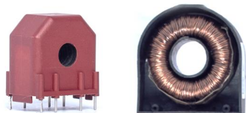
Figure 2. General view PCB mounded products
