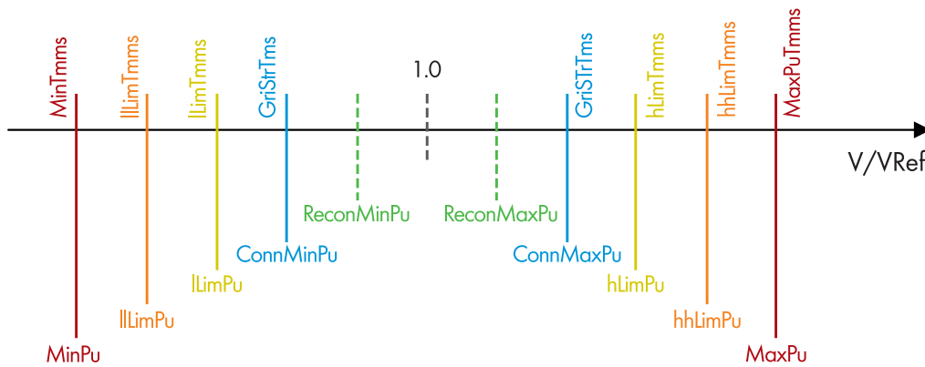
Figure 18: Voltage monitoring
